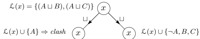
Figure 7: Semantic branching search
